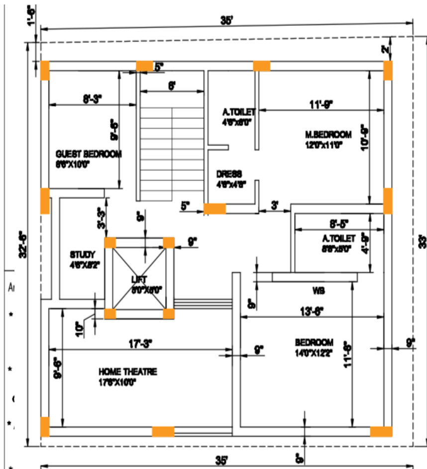
PROPOSED THIRD FLOOR PLAN
